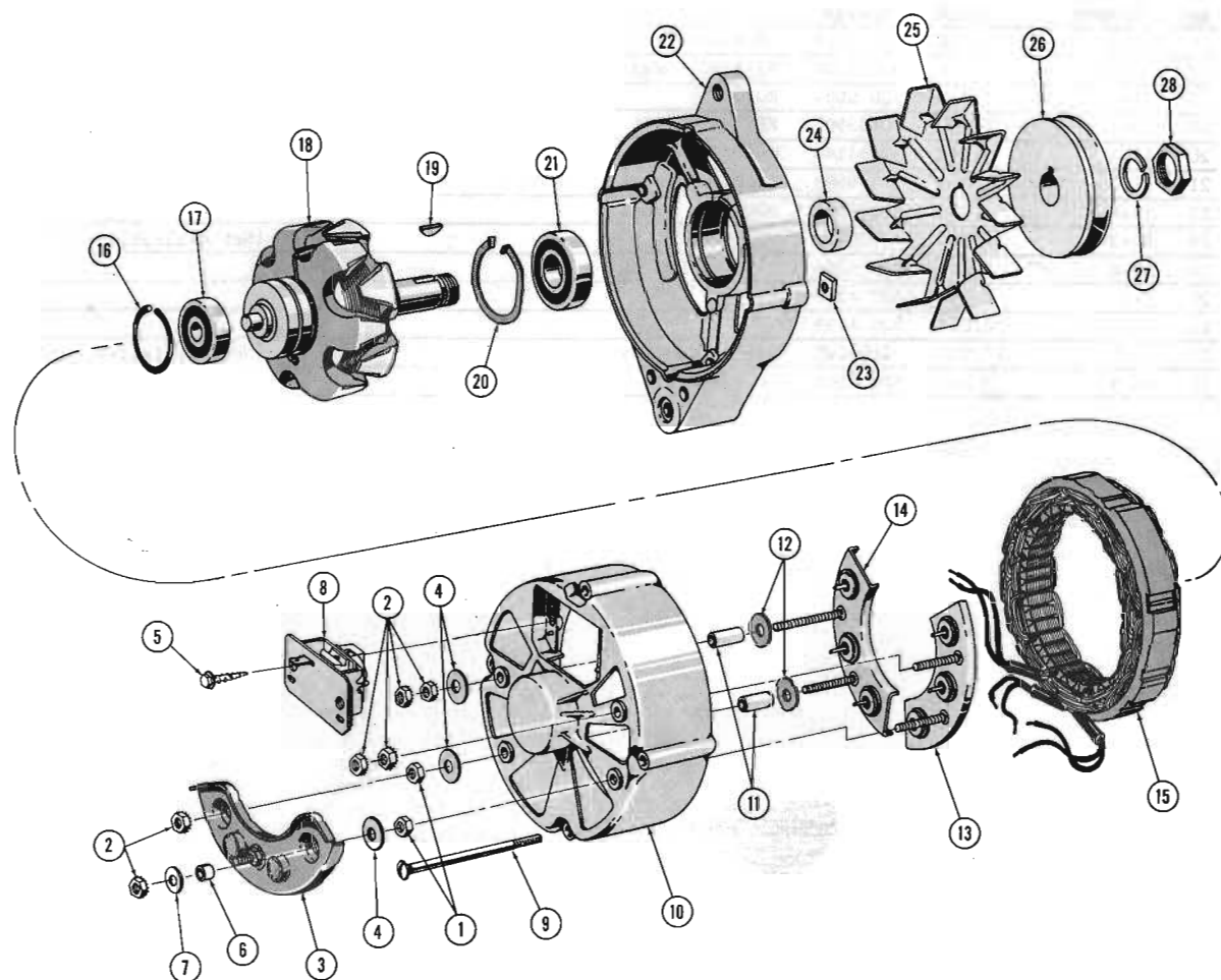
ALTERNATOR (Less Pulley and Belt)(40 AMP.) 64-65 01-10-80
