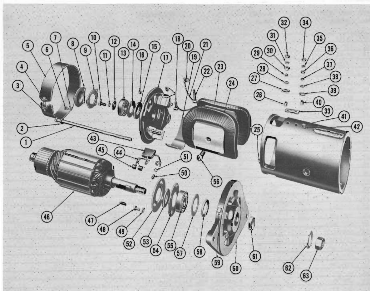
GENERATOR 60 THRU 62 01-10: 60-61 20-80 (40 AMP.)(LOW CUT IN)(REFER NOTE 3.005-4)
