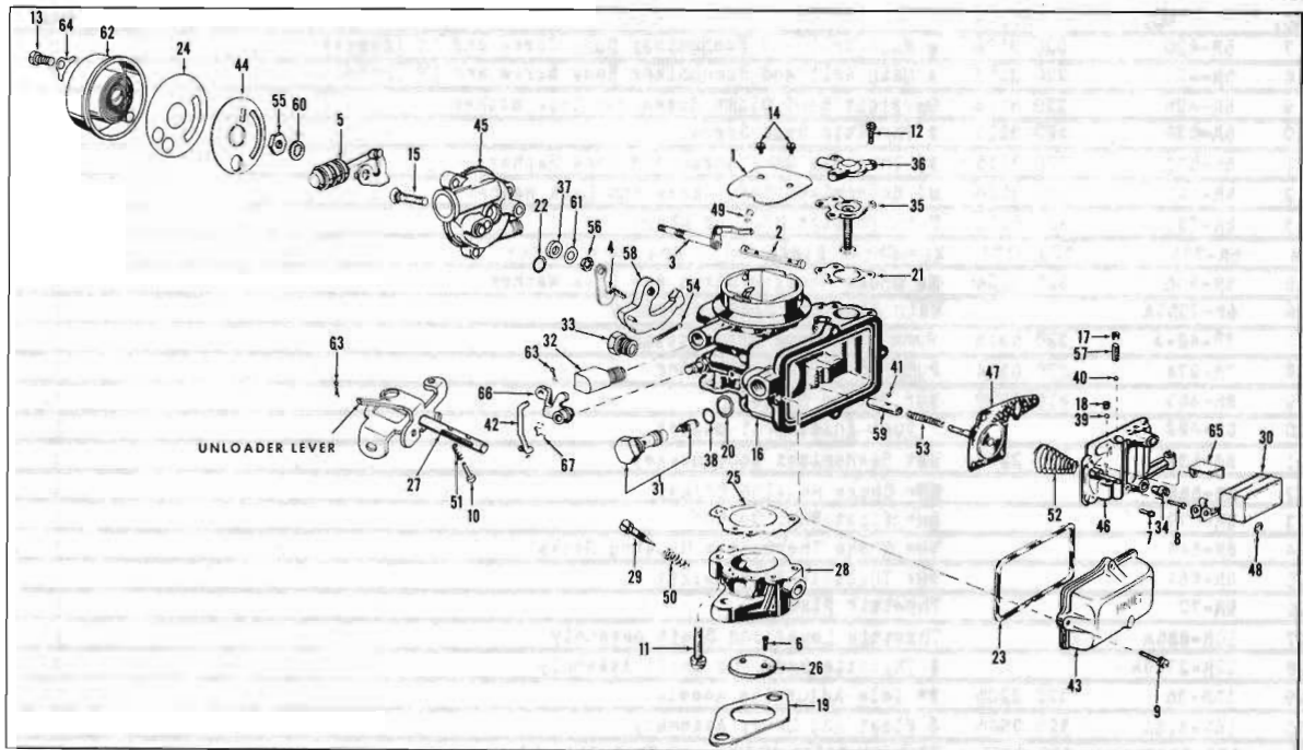
CARBURETOR 61-62 10 (WST-LDT)(WOD-LDT)
